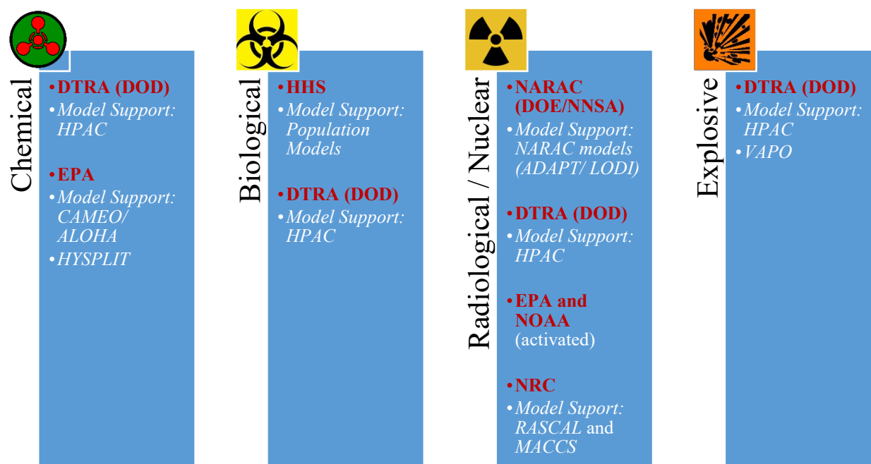
Figure 1: Summary of IMAAC’s agency responsibilities with the typical dispersion model used, based on information from DTRA (Runyon 2017).
