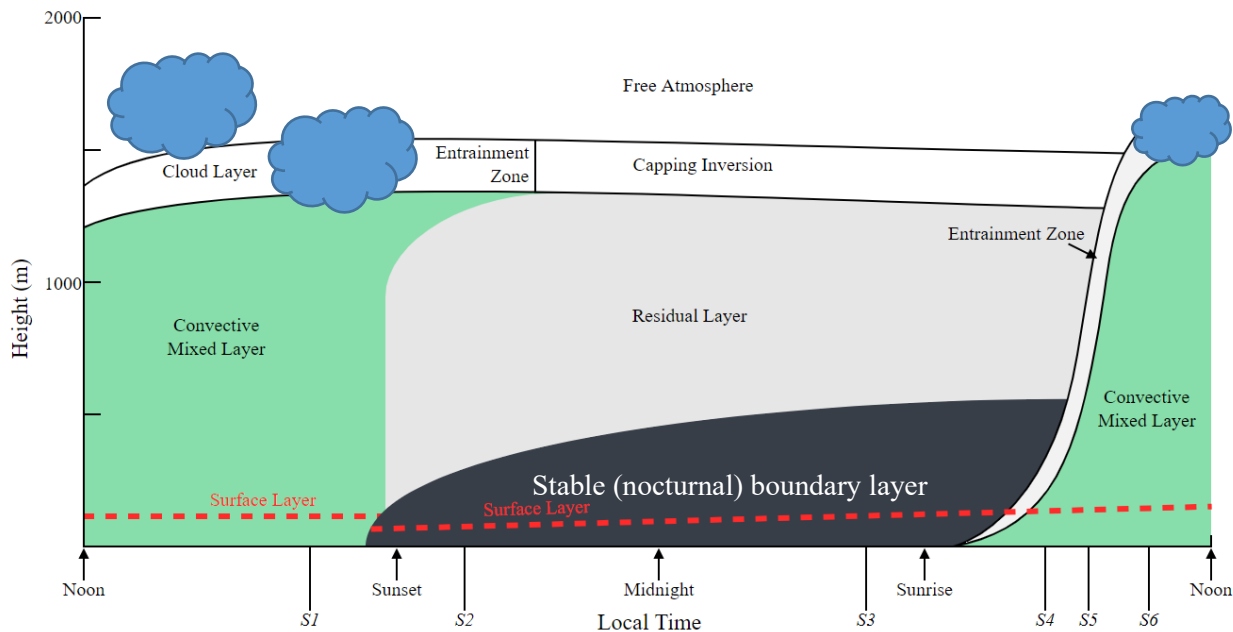
Figure 2: The common, but idealized, diurnal evolution of the Planetary Boundary Layer (PBL) adapted from Stull (1988).
