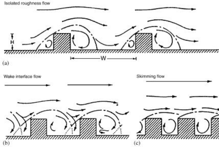
Figure 5: Various perpendicular flows for urban canyons with a) isolated roughness, b) wake interference, and c) skimming flow aspect ratios, based on Oke (1988).
