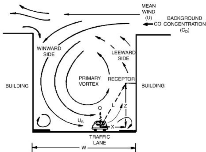
Figure 4: Schematic of streamlines when perpendicular flow encounters a street canyon, based on Dabberdt et al. (1973).
