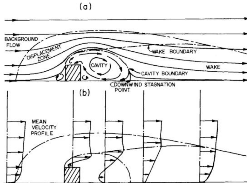
Figure 3: Schematic of a) cavity and wake flow zones associated with a building or other square obstacle in the mean flow and b) its relationship with the vertical wind profile, after Halitsky (1968).
