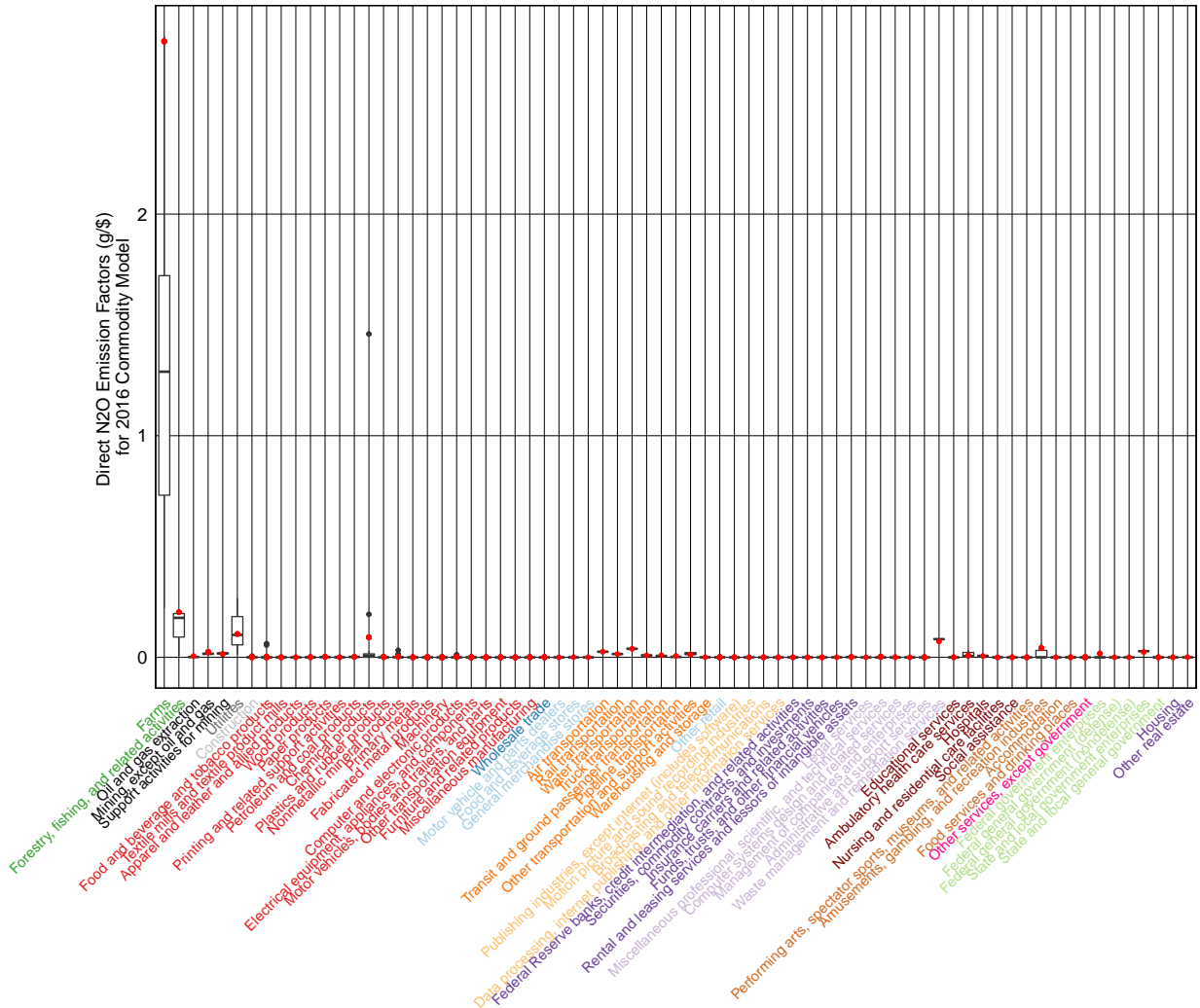
Figure A8 - 3: Nitrous oxide direct emission factors: summary level commodities (red dots) compared to detail level commodities (box plots) in 2016.
