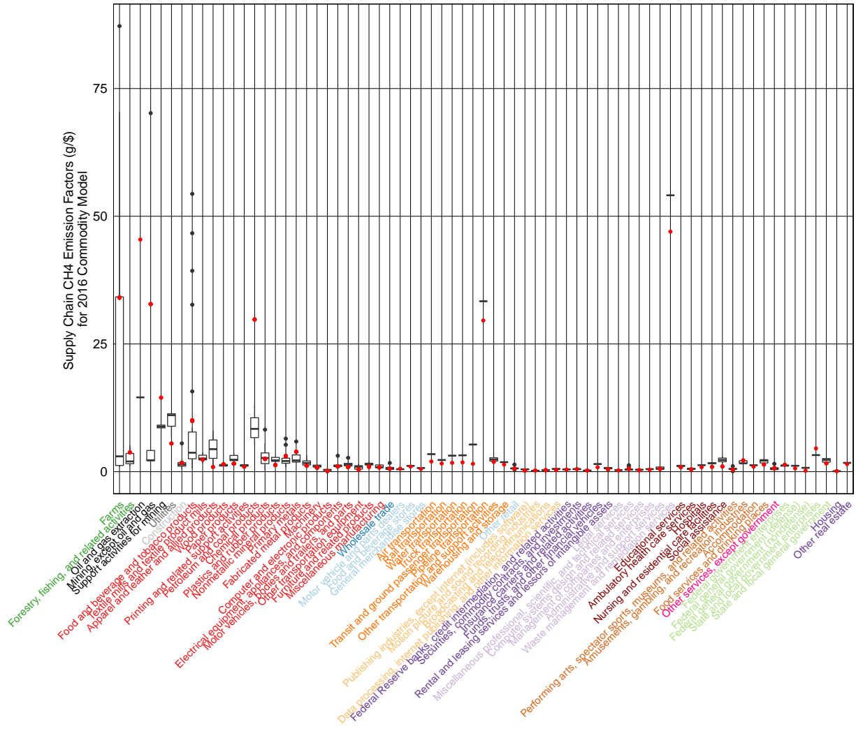
Figure A8 - 5: Methane supply chain emission factors: summary level commodities (red dots) compared to detail level commodities (box plots) in 2016.
