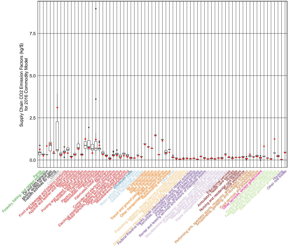
Figure A8 - 4: Carbon dioxide supply chain emission factors: summary level commodities (red dots) compared to detail level commodities (box plots) in 2016.
