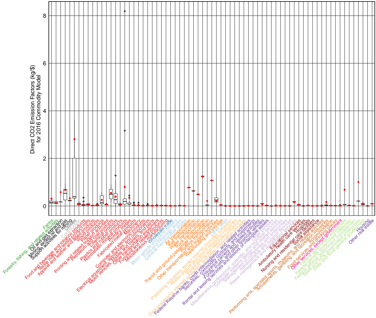
Figure A8 - 1: Carbon dioxide direct emission factors: summary level commodities (red dots) compared to detail level commodities (box plots) in 2016.
