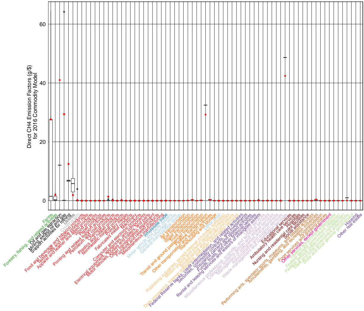
Figure A8 - 2: Methane direct emission factors: summary level commodities (red dots) compared to detail level commodities (box plots) in 2016.
