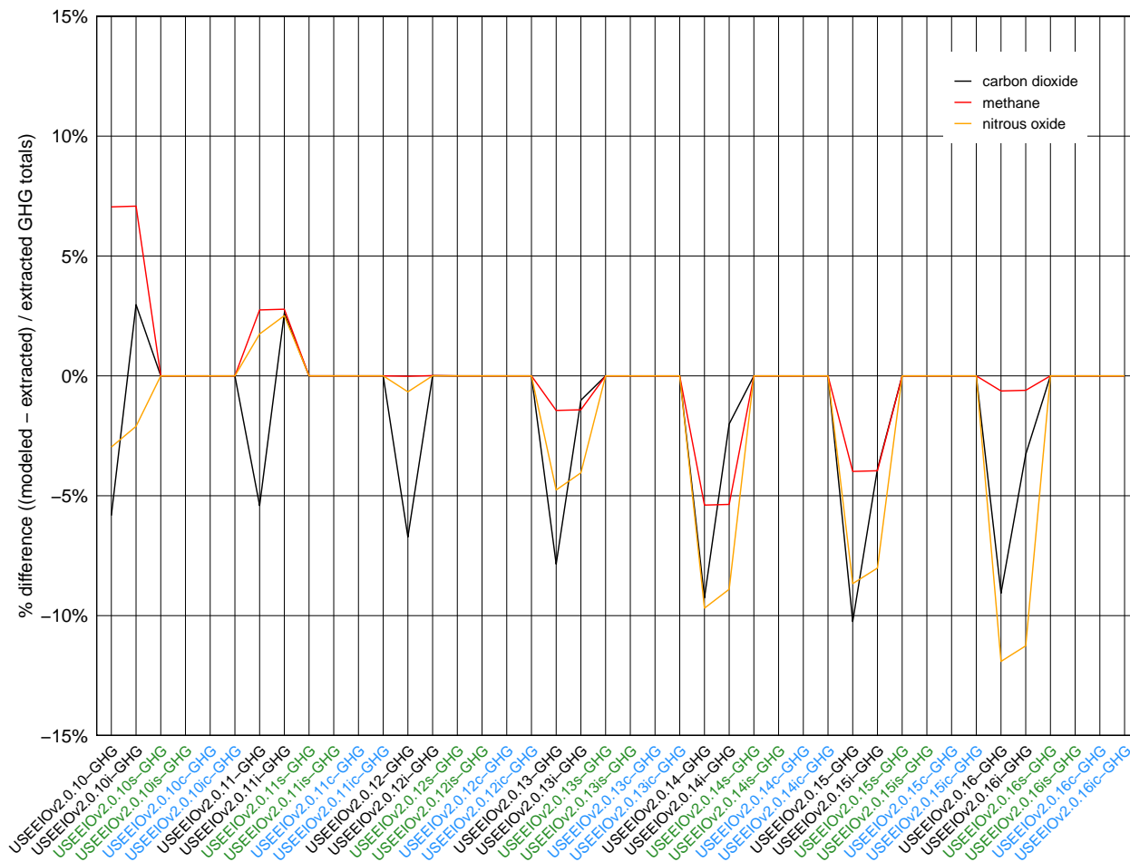
Figure A10 - 1: National GHG validation totals
