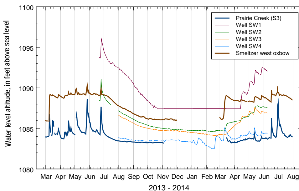
Figure 6. Altitude of water level in groundwater and the Smeltzer west oxbow wetland.
