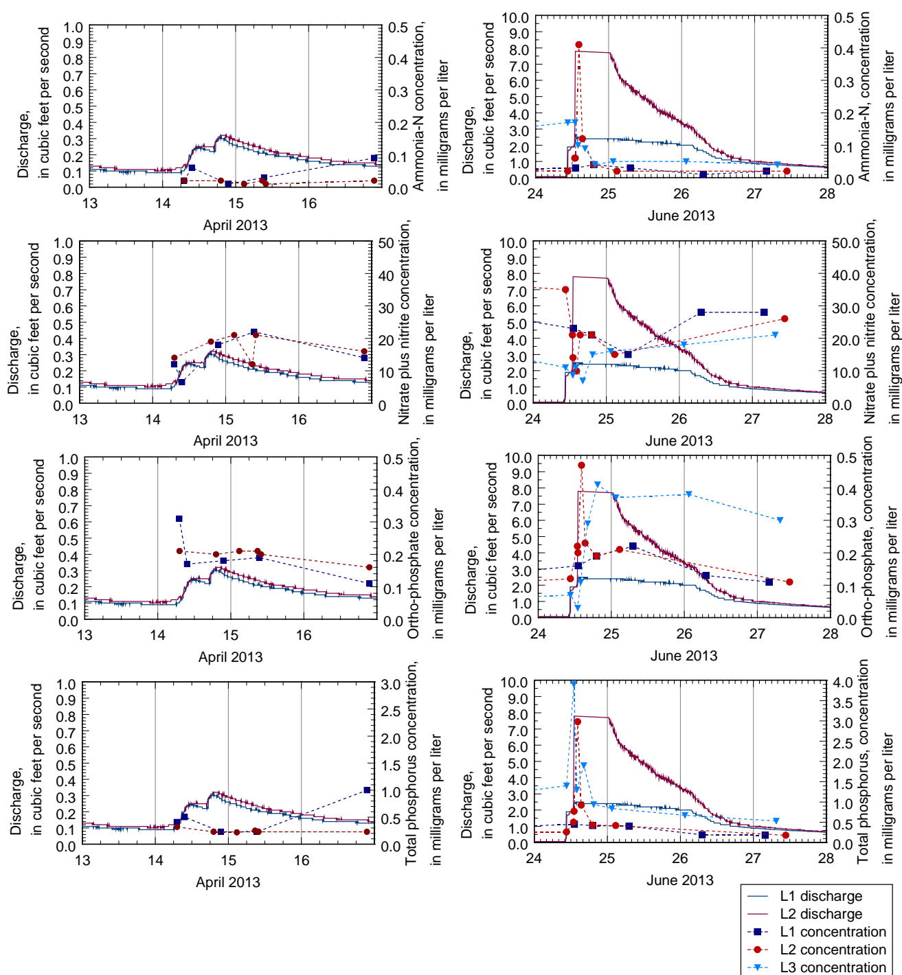
Figure 11. Flow and concentrations of selected nitrogen and phosphorus species in tile line inflow (L1) and discharge from (L2) the Lyons Creek oxbow wetland during two storm events in 2013.
