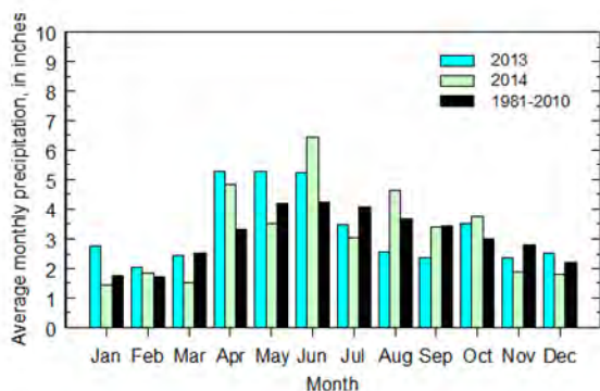
Figure 4. Average monthly air temperature and precipitation in central Iowa in 2013 and 2014 in relation to the 30-year average. (monthly summary of the entire Iowa climatic region 5; data from NOAA, 2015)
