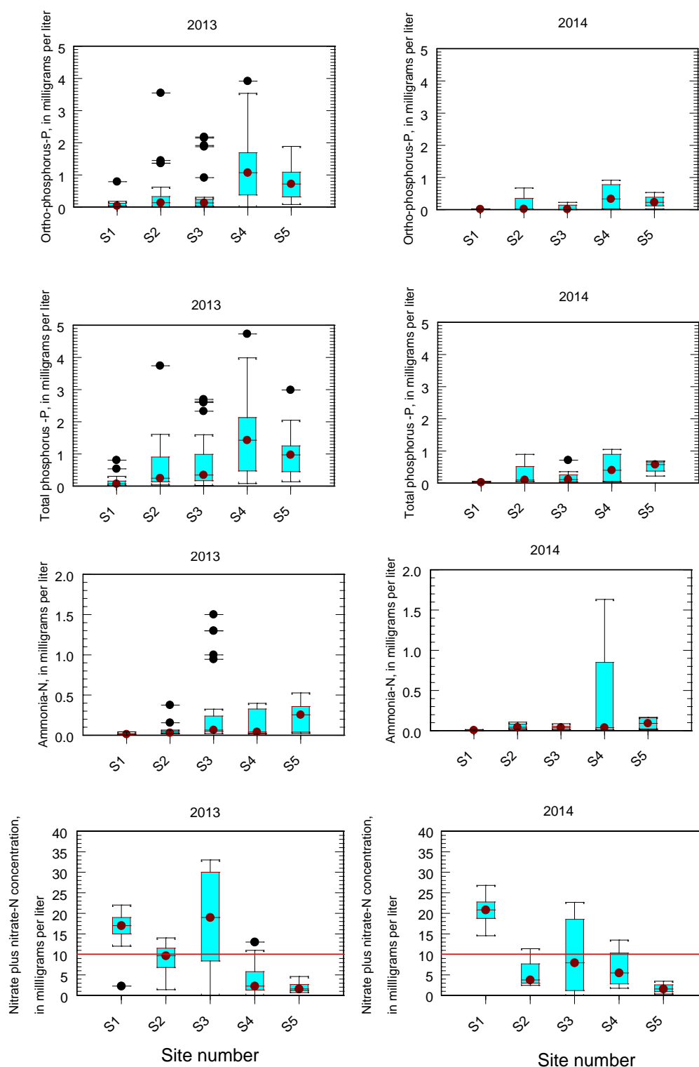
Figure 9. Summary of concentrations of selected phosphorus and nitrogen species at the Prairie Creek study site, 2013-2014. [The horizontal red line is the drinking water standard. It is supplied for a perspective as to how much the nutrient concentrations in the water would need to be reduced by water treatment to be consumed as drinking water. Iowa does not currently have numeric criteria for surface water nutrients.]
