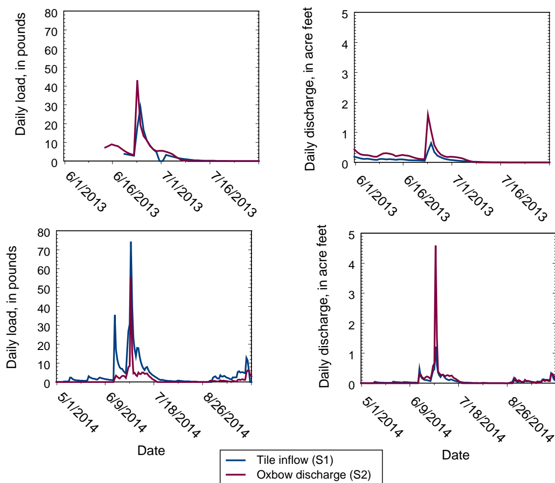
Figure 17.—Daily Inflow from a tile line (S1) and outflow (S2) of water and nitrate from the Smeltzer west reconstructed oxbow wetland,
