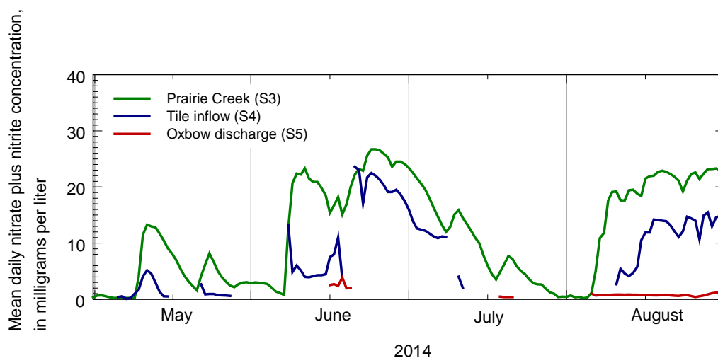
Figure 15. Daily mean nitrate plus nitrite concentration in Smeltzer east oxbow wetland inflow (S4), outflow (S5), and in the receiving stream, Prairie Creek (S3)
