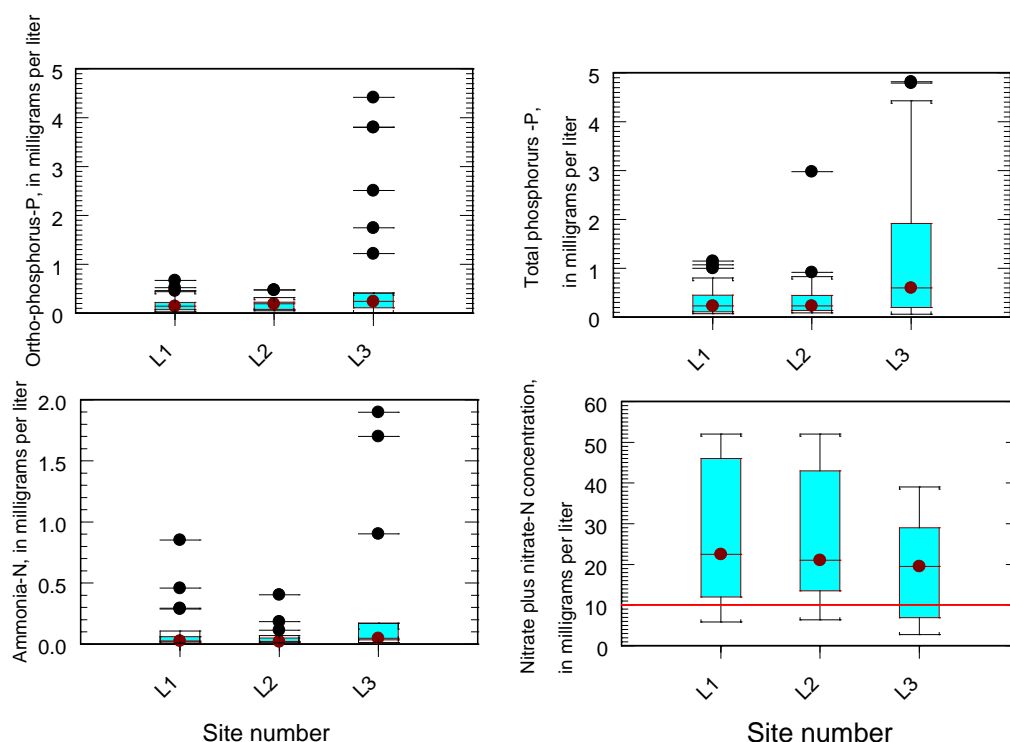
Figure 8. Summary of concentrations of selected phosphorus and nitrogen species at the Lyons Creek study site, 2013
