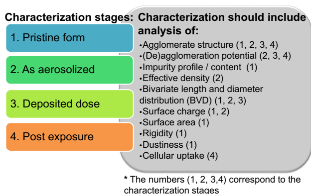
Fig. 4 NMs characterization during the course of a study. Ideally, NMs will be characterized in their original dry form, as aerosolized, as deposited, and at multiple time points during the course of the study. The characterization conducted will depend on the stage of the NM [i.e., (1) pristine form; (2) as aerosolized; (3) deposited dose; and (4) post-exposure] and, in this figure, the numbers 1 through 4 in parentheses following each parameter correspond to the four stages of NMs listed
