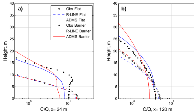
Figure 5. Vertical profiles of concentration measured in the wind tunnel and simulated with two models at full scale downwind distances of a) x = 24 m, and b) x = 120 m.
