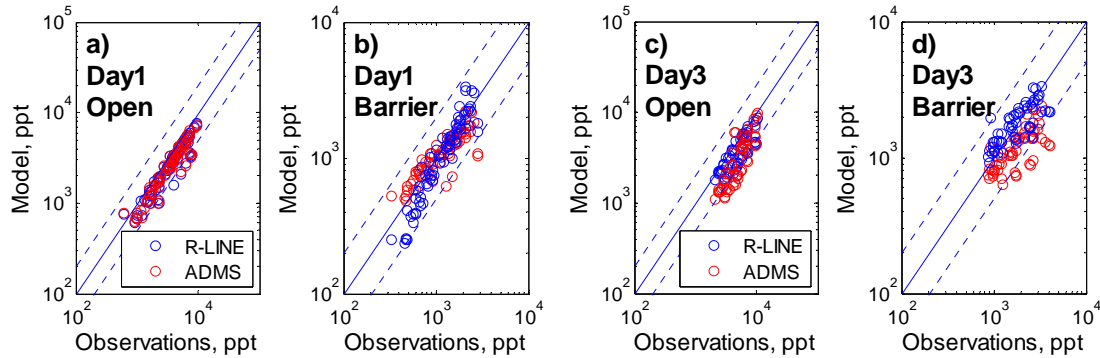
Figure 3. Idaho Falls results showing scatter plots of the average of the lateral peak concentrations with the neighbouring concentrations at each downwind distance for each 15 minutes period considered. Plots a & b show results for the day with neutral atmospheric conditions (open terrain and with barrier, respectively); similarly c & d for the weakly stable day. The solid and dashed lines are the 1:1 and factor of two lines, respectively.
