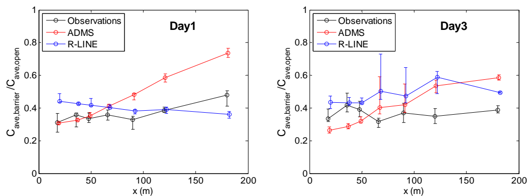
Figure 2. Results for the neutral (Day 1) and weakly stable (Day 3) test periods. Plots show the ratio of average concentrations with the barrier to those measured in open terrain. The “error bars” correspond to 25 th and 75 th percentile and circle is at the median.
