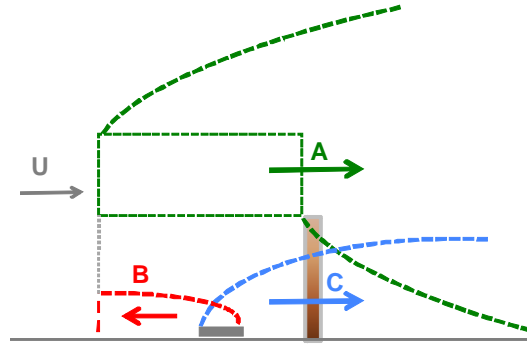
Figure 1. Illustration of the main component sources used in the ADMS-Urban advanced street canyon module for a noise barrier configuration.
