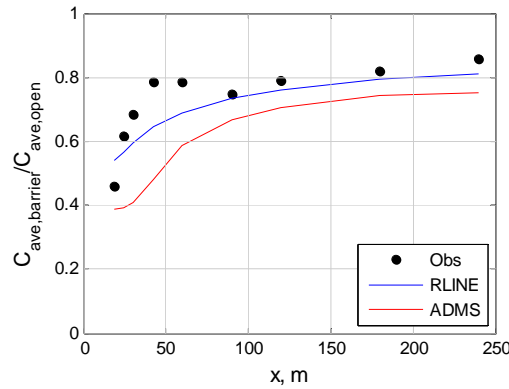
Figure 4. Observed and modelled ratios of the average concentrations with a barrier to those in open terrain for the wind tunnel experiment.
