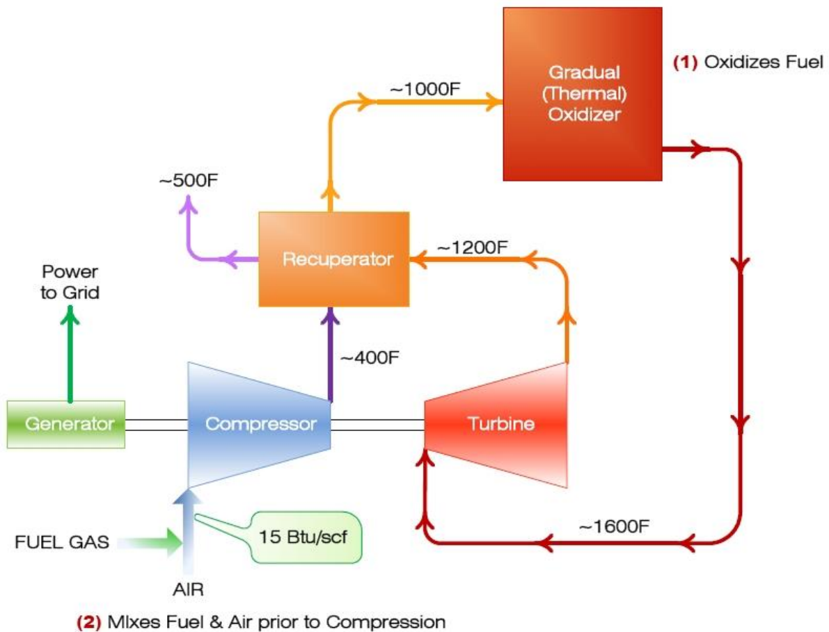
Figure 1. Flex Powerstation Schematic
