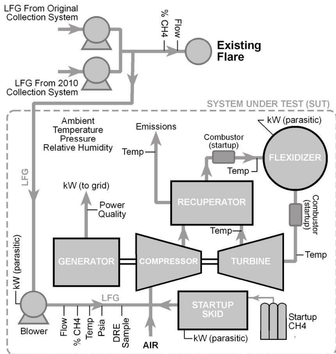
Figure 6. Flex System Monitoring Schematic
