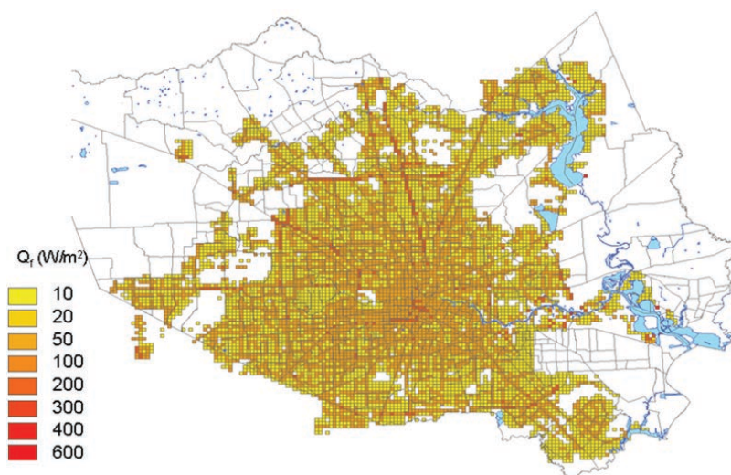
FIG. 4. Example of maximum AH fluxes ( Q_t ) gridded at 500 m on an hourly basis in NUDAPT, based on the method by Sailor and Lu (2004). Example shown is for Houston, TX, for a “typical” day at 2000 UTC in Aug.
