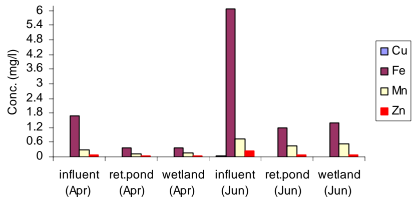
Figure 13. Concentrations of heavy metals in the influent (runoff) and mesocosm effluents
