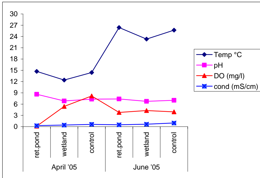
Figure 7. YSI monitoring in retention pond and wetland mesocosms
