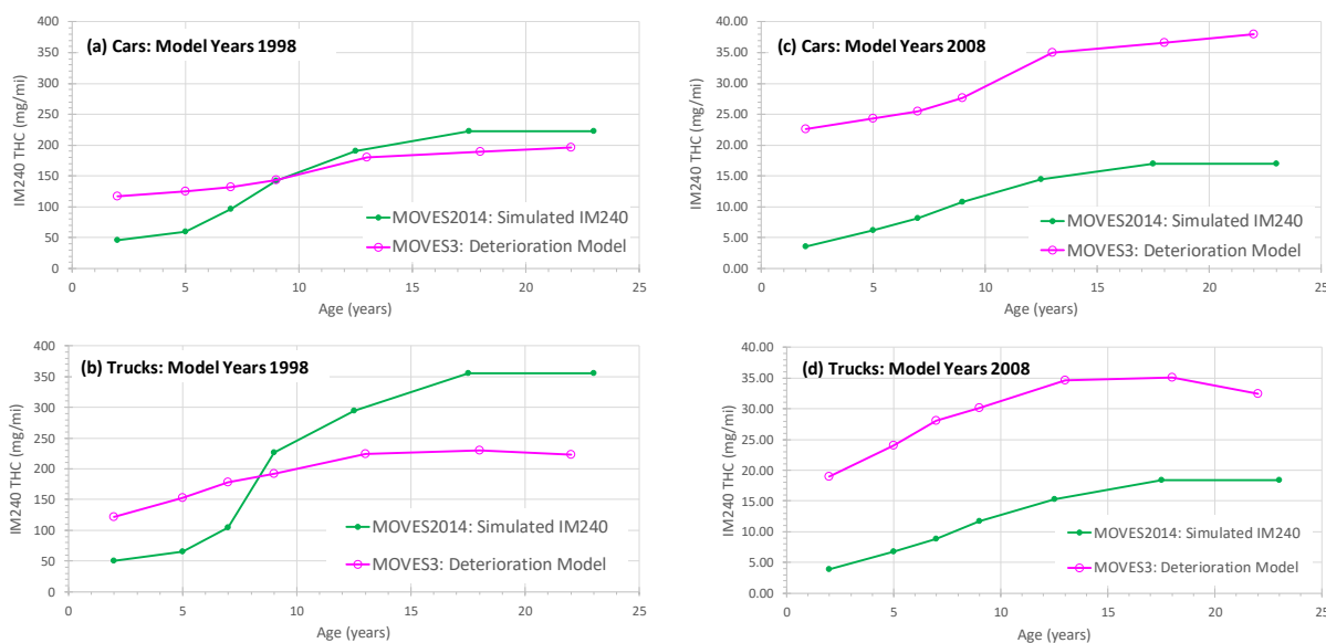
Figure 3-71 THC: Predicted trends in IM240 emissions vs age for cars and trucks in two model years
