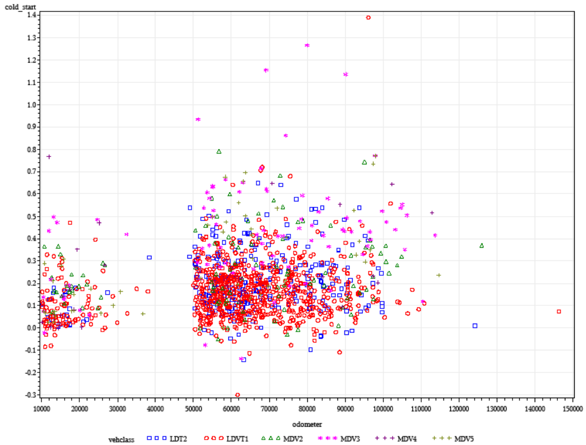
Figure 3-97 Cold-start FTP emissions for NO x (g) vs. odometer (mi), for LEV and ULEV vehicles, from the IUVF program
