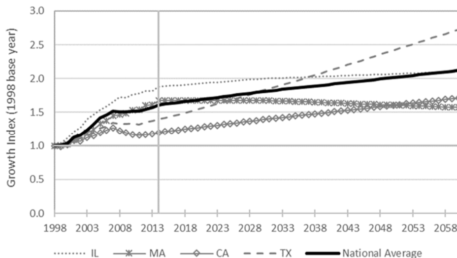
Figure 4.4 Annual growth indices from 1998 base year to 2060 for Commercial Lawn and Garden equipment. The vertical line at 2014 indicates the transition between historical and projection indices.
