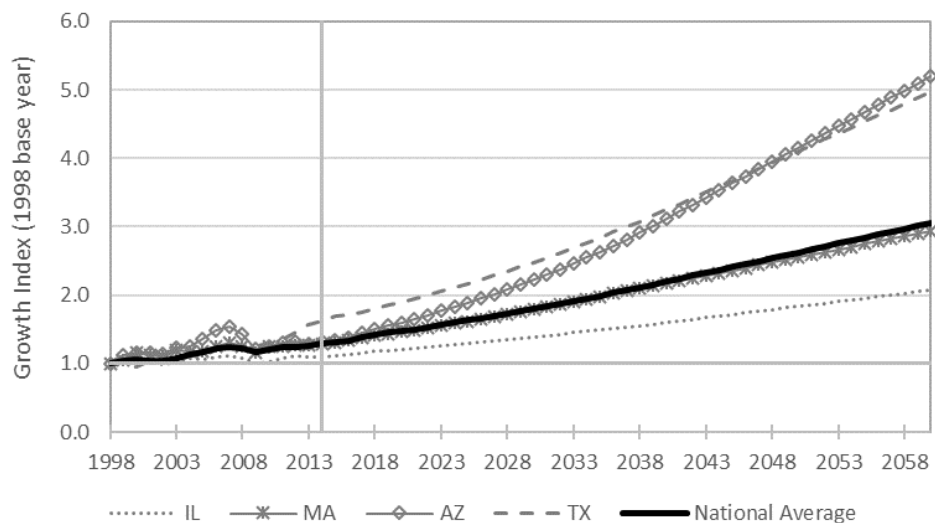
Figure 4.2 Annual growth indices from 1998 base year to 2060 for Commercial equipment. The vertical line at 2014 indicates the transition between historical and projection indices.
