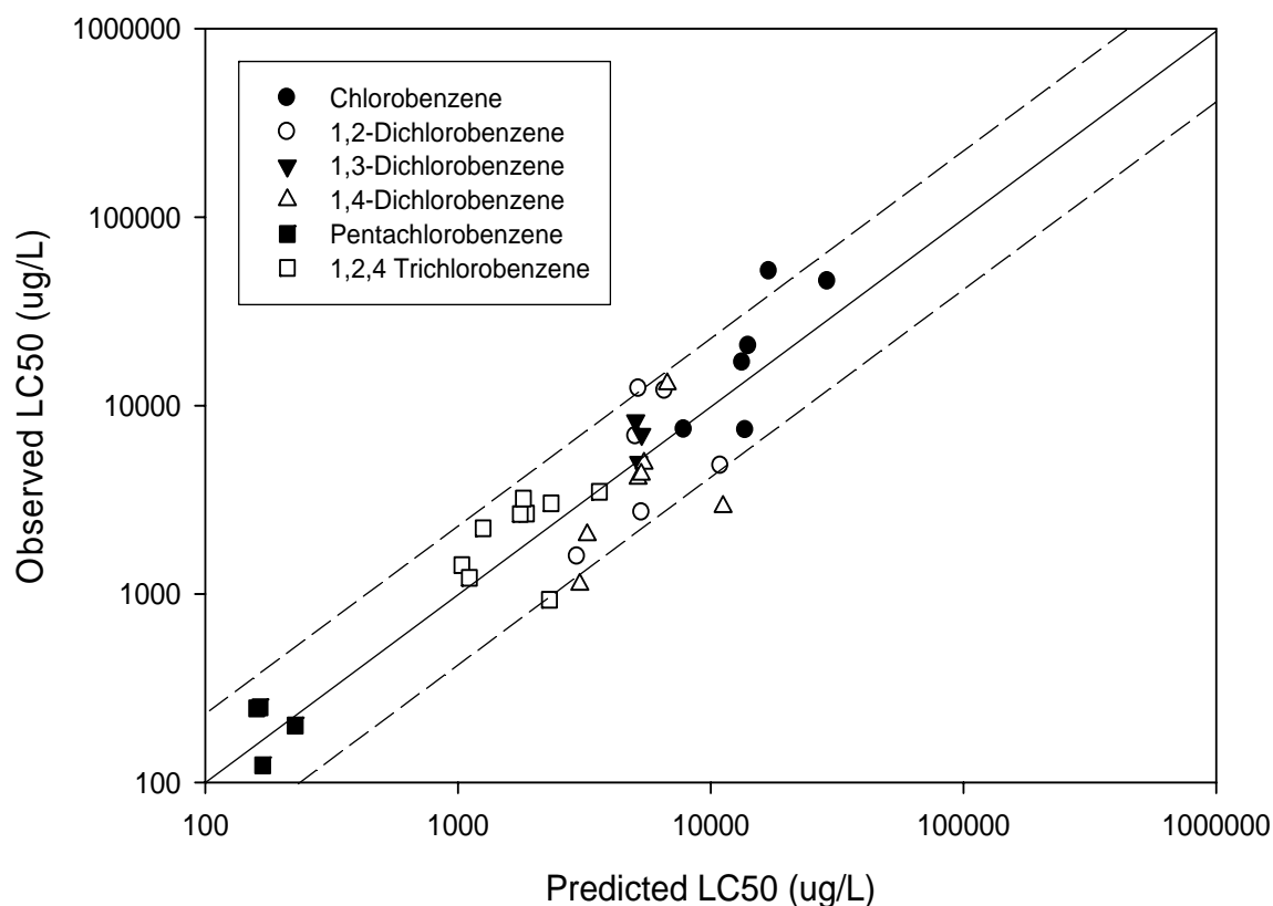
Figure 2-4 Comparison of observed LC_{50} values used in the calculation of secondary chronic values and LC_{50} values predicted using narcosis theory as described by Di Toro et al. (2000) for chlorobenzenes (including Chaisuksant et al. (1998)). Plot shows data for all species that had both measured LC_{50} data in the SCV derivation and have species-specific sensitivity data as calculated by Di Toro et al. (2000). See discussion in text for more details. The solid line is the one to one line and the dashed lines show \pm a factor of two.
