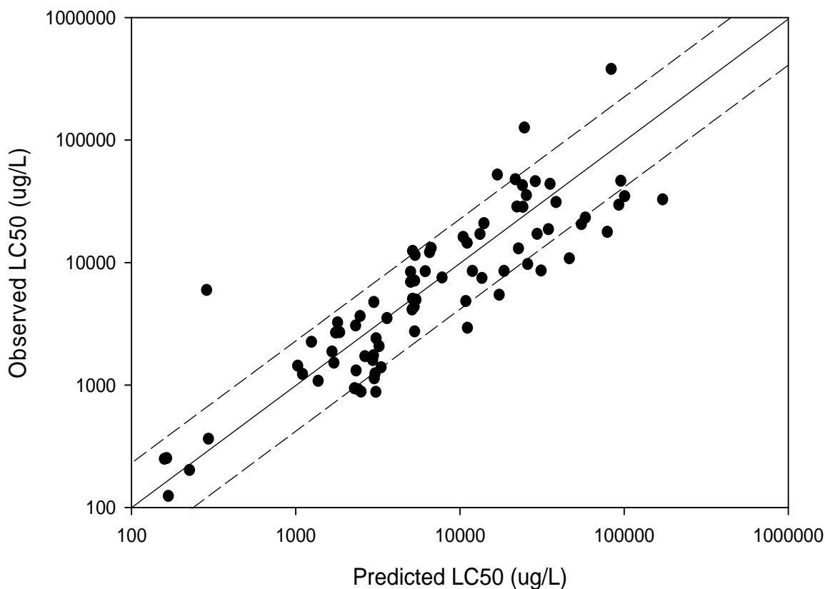
Figure 2-2 Comparison of observed LC 50 values used in the calculation of secondary chronic values and LC 50 values predicted using narcosis theory as described by Di Toro et al. (2000) for all 20 narcotic chemicals discussed in this document (including data from Chaisuksant et al. (1998)). Plot shows data for all species that had both measured LC 50 values in the SCV derivation and have species-specific sensitivity data as calculated by Di Toro et al. (2000). See discussion in text for more details. The solid line is the one to one line and the dashed lines show \pm a factor of two. Chemicals potentially having more specific modes of action (e.g., pesticides and phthalates) are not shown.
