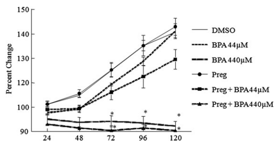
FIG. 4. Effect of pregnenolone cotreatment with BPA on antral follicle growth. Antral follicles were mechanically isolated from FVB mice and exposed in vitro to BPA (4.4–440 μM), pregnenolone (10 μg/ml) or pregnenolone, and BPA (44–440 μM) for 120 h. Growth of follicles was monitored during culture and recorded in micrometers and reported as percent change. The graph represents means ± SEMs from at least three separate experiments. Lines with asterisks (*) are significantly different from DMSO controls ( n = 8\text{--}16 follicles per treatment per experiment from at least three separate experiments; p \leq 0.05 ).
