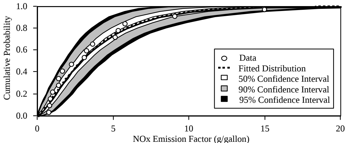
Figure 1. Fitted Gamma Distribution and Bootstrap Simulation Results for 2-Stroke Lawn and Garden Engine NO x Emission Data in Units of g/gallon (n=16).
