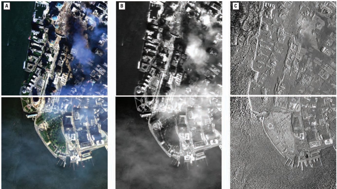
Figure 5. AVIRIS imagery of lower Manhattan acquired on 16 September 2001. (A) Visible color composite of the plume (RGB = 0.66/0.55/0.44 \mu\text{m} ). (B) The short-wavelength visible blue band (0.44 \mu\text{m} ) shows the extent of aerosol scattering as brighter areas. (C) The near-infrared band ratio (0.94 \mu\text{m} /0.86 \mu\text{m} ) indicates the spatial extent of the plume.
