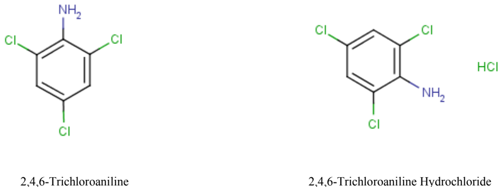
Figure 1. Chemical Structures of 2,4,6-Trichloroaniline and 2,4,6-Trichloroaniline Hydrochloride
