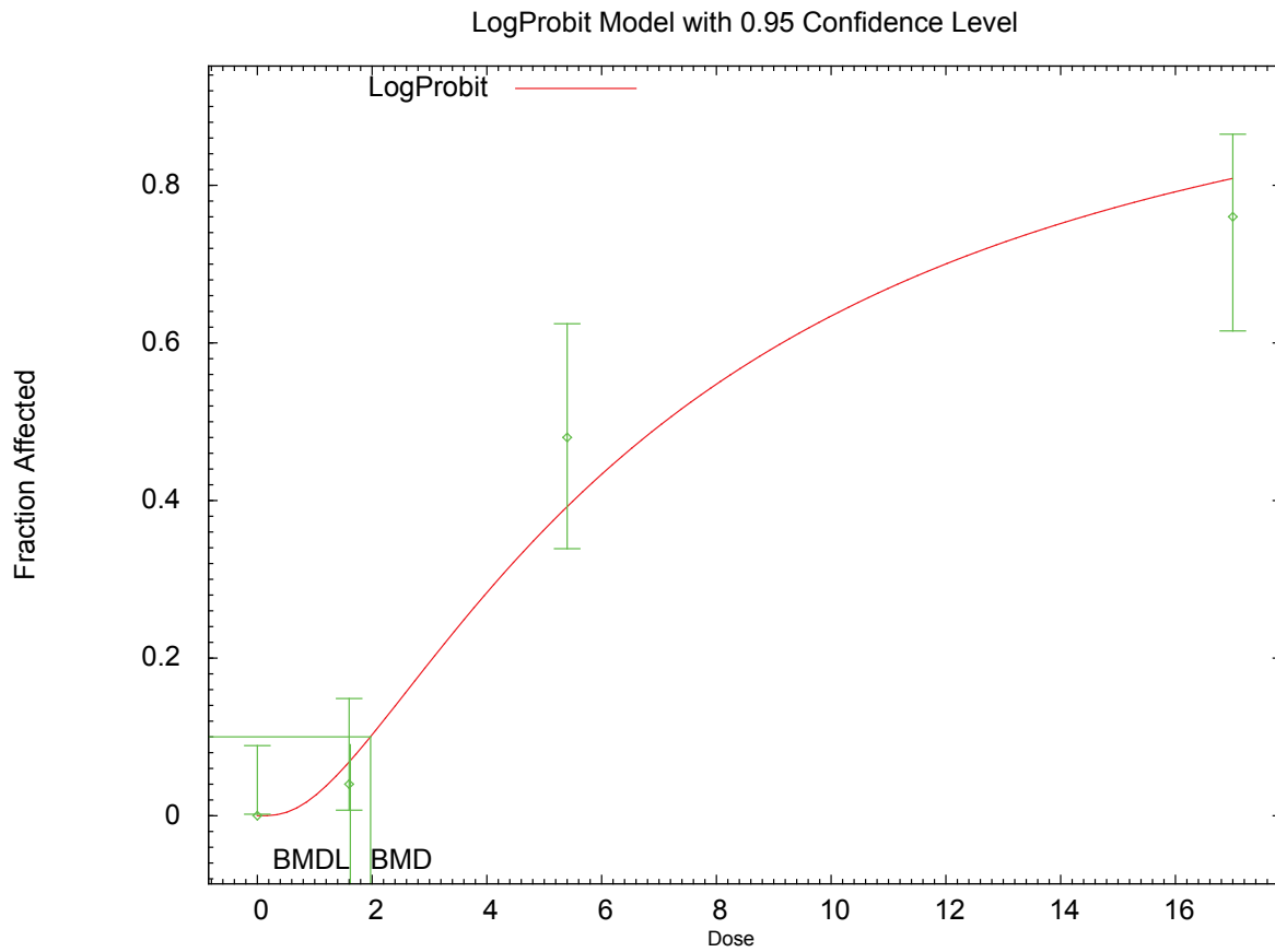
Figure B-1. Fit of Log Probit Model to Data on Centrilobular Hypertrophy (NTP, 2001)
