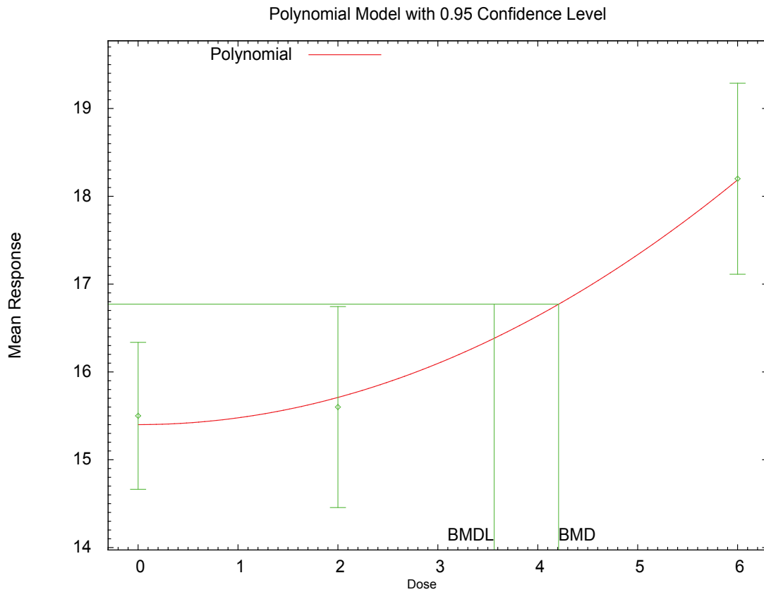
Figure A-1. Fit of 2-Degree Polynomial (Constant Variance) Model to Data for Changes in Absolute Liver Weight in Male Rats (NTP, 2001)
