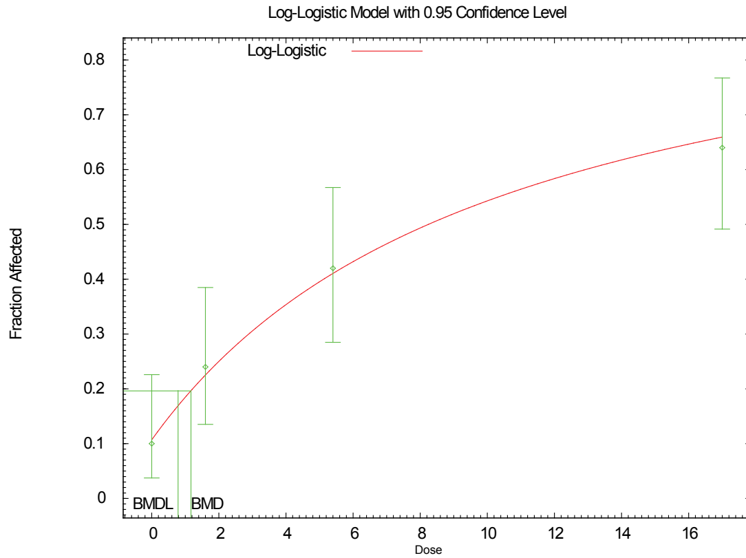
Figure B-2. Fit of Log-Logistic Model to Data on Bile-Duct Hyperplasia (NTP, 2001)
