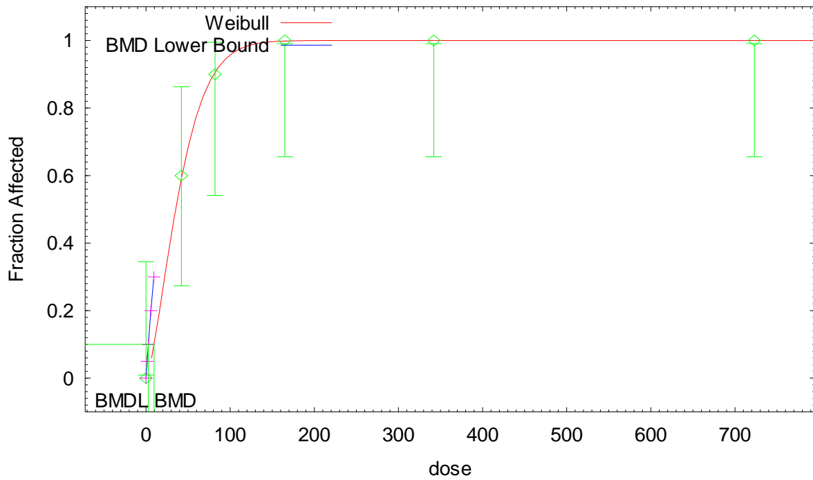
Weibull Model with 0.95 Confidence Level
