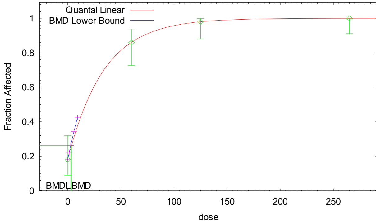
Quantal Linear Model with 0.95 Confidence Level
