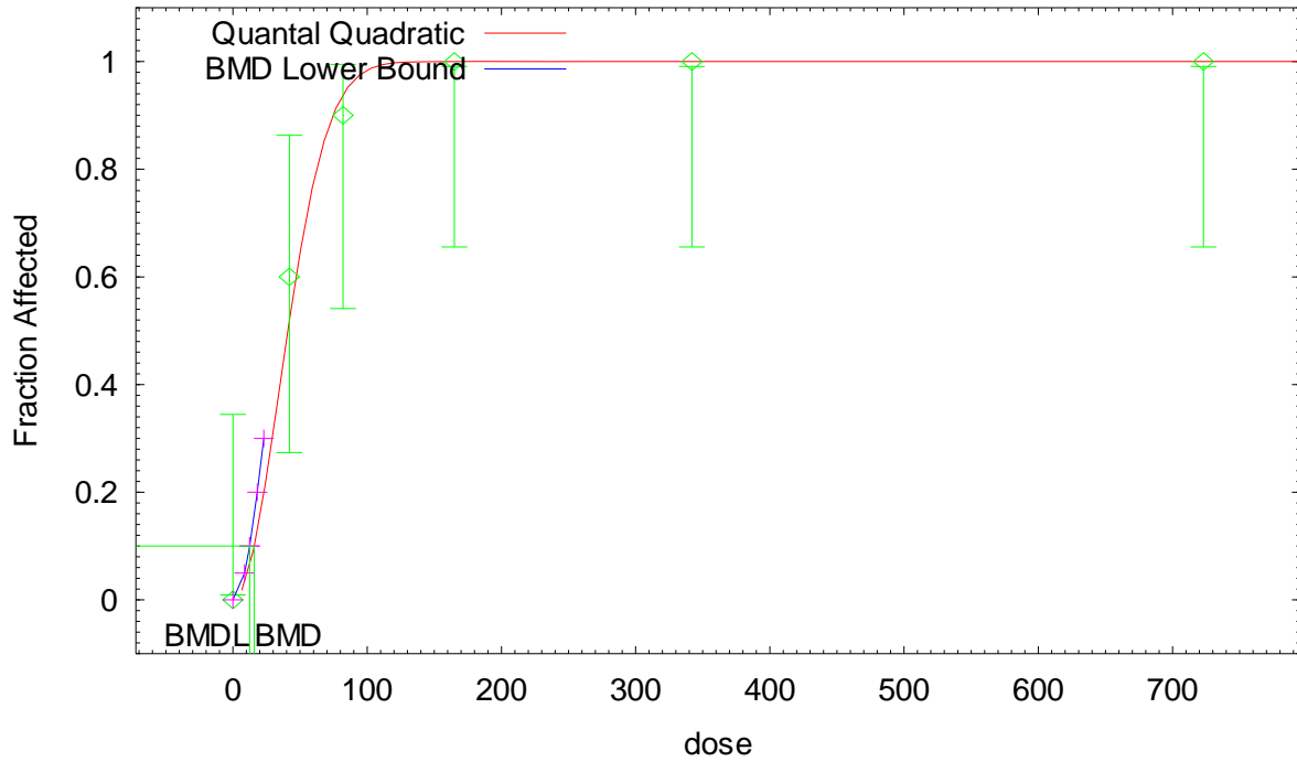
Quantal Quadratic Model with 0.95 Confidence Level
