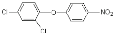
Figure 1. Nitrofen Structure
