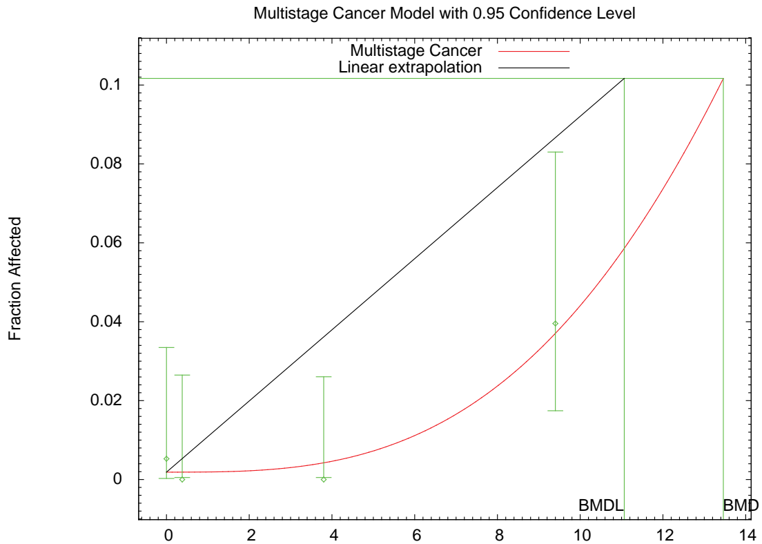
Figure C-3. Fit of Multistage Cancer, 3-Degree Model to Data on Nasal Adenoma in Male Hamsters Exposed to Methyl Hydrazine by Inhalation for 1 Year (Kinkead et al. (1985)).
