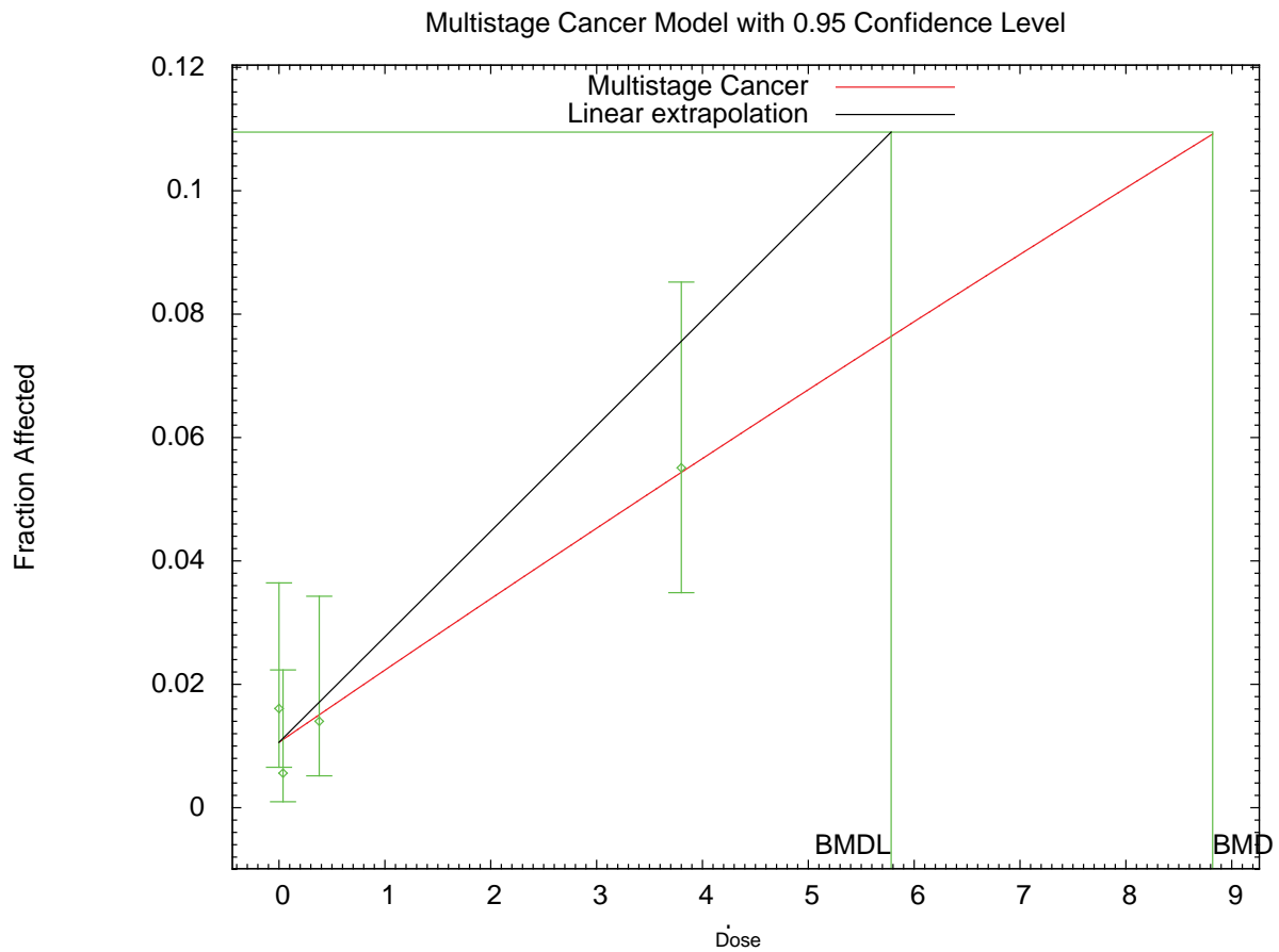
Figure C-2. Fit of Multistage Cancer, 1-Degree Model to Data on Liver Adenoma in Female Mice Exposed to Methyl Hydrazine by Inhalation for 1 Year (Kinkead et al. 1985).
