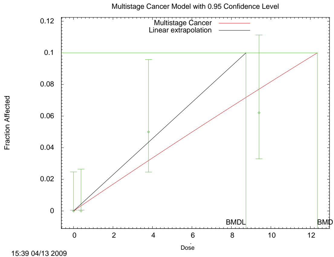
Figure C-4. Fit of Multistage Cancer, 1-Degree Model to Data on Nasal Adenomatous Polyps in Male Hamsters Exposed to Methyl Hydrazine by Inhalation for 1 Year (Kinkead et al., 1985).
