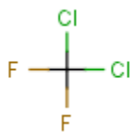
Figure 1. Chemical Structure of Dichlorodifluoromethane
