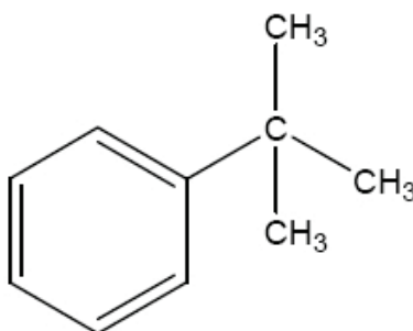
Figure 1. tert -Butylbenzene Structure
