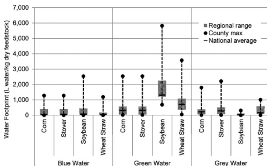
Figure 23 An estimate of the blue, green and grey water footprint associated with corn grain, stover, wheat straw and soybean during the crop growing phase. The national production-weighted average is represented by the horizontal bar, while the regional ranges (USDA regions including the Corn Belt, Southern Plains, etc.) are represented by the shaded bars. County-level variation in feedstock water footprints, shown in dashed lines, are driven by differences in irrigation and evapotranspiration (ET). [Source: Chiu and Wu (2012)].
