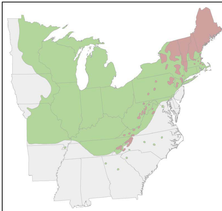
Figure 5-4 Distribution of Red Spruce (pink) and Sugar Maple (green) in the Eastern U.S. 94
