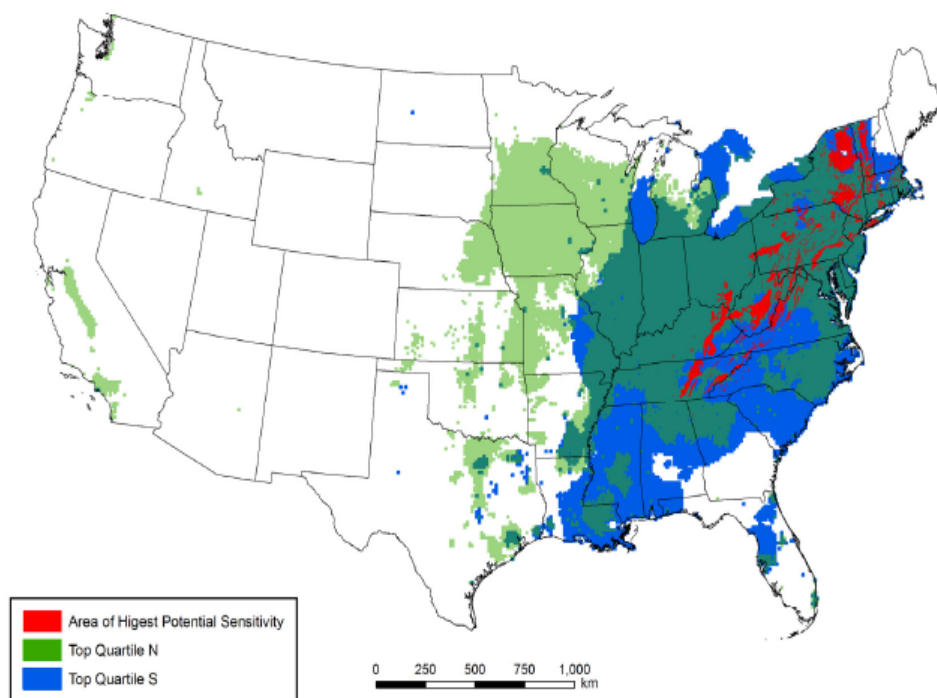
Figure 5-3 Areas Potentially Sensitive to Terrestrial Acidification
