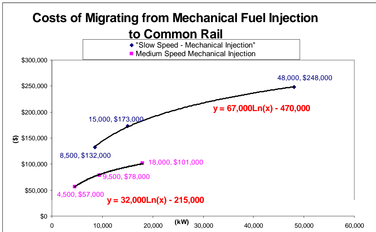
Figure 6-5 Variable Cost Curve-Fit for Mechanically Controlled MFI to Common Rail Fuel Injection Systems
