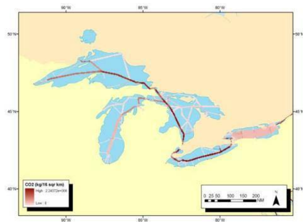
Figure 4-2 Illustration of STEEM Modeling Domain and Spatial Distribution of Shipping Lanes
