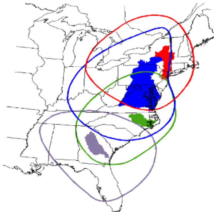
Figure 5-2 Principal Airsheds and Watersheds for Oxides of Nitrogen for Estuaries. Hudson/Raritan Bay; Chesapeake Bay; Pamlico Sound; and Altamaha Sound (listed from north to south)
