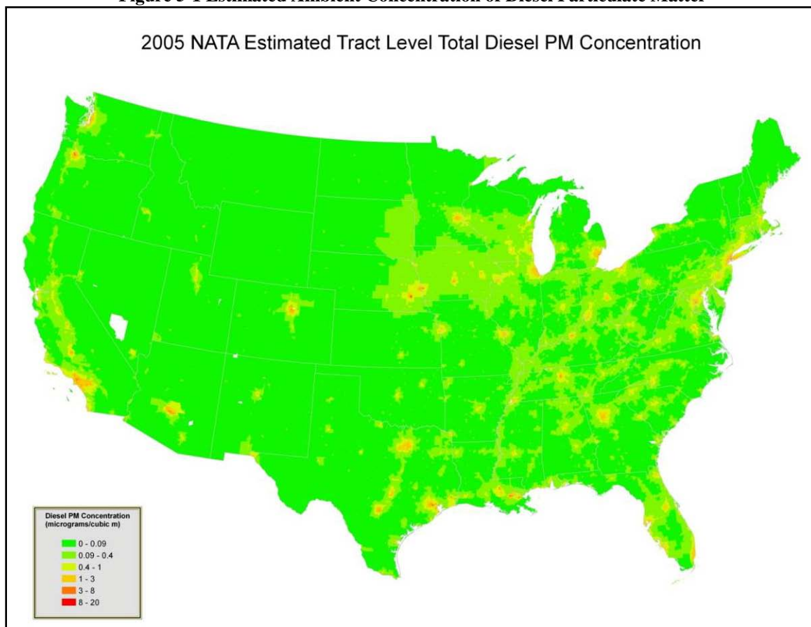
Figure 5-1 Estimated Ambient Concentration of Diesel Particulate Matter
