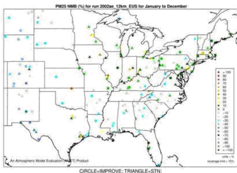
Figure 5A-4 Normalized Mean Bias (%) of annual PM_{2.5} by monitor for 12-km Eastern U.S. domain, 2002
