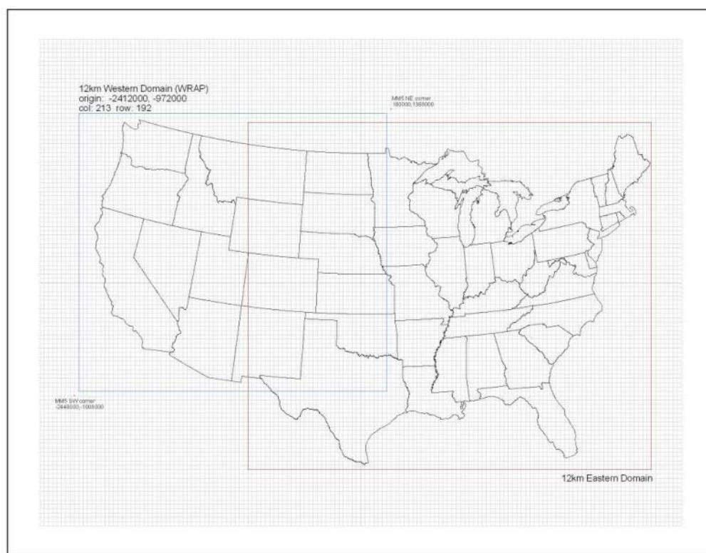
Figure 5A-1 Map of the CMAQ Modeling Domain
