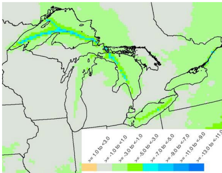
Figure 5-13 Percent Change in Annual Total Sulfur Deposition in 2020 from the Coordinated Strategy
