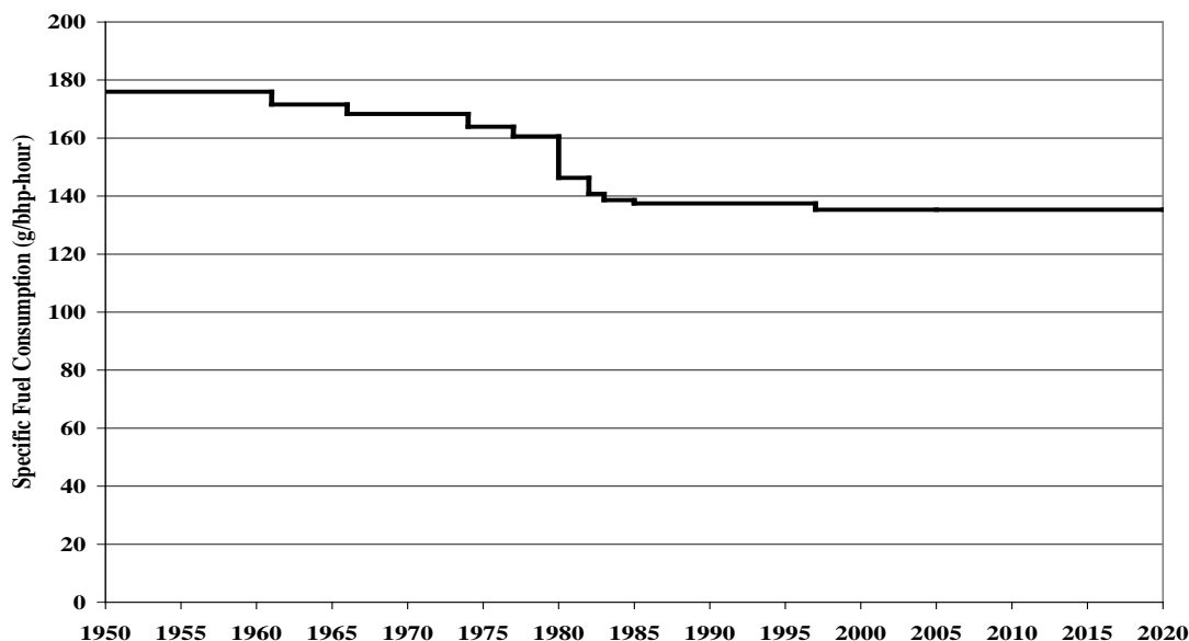
Figure 4D--3 Diesel Engine Specific Fuel Consumption
