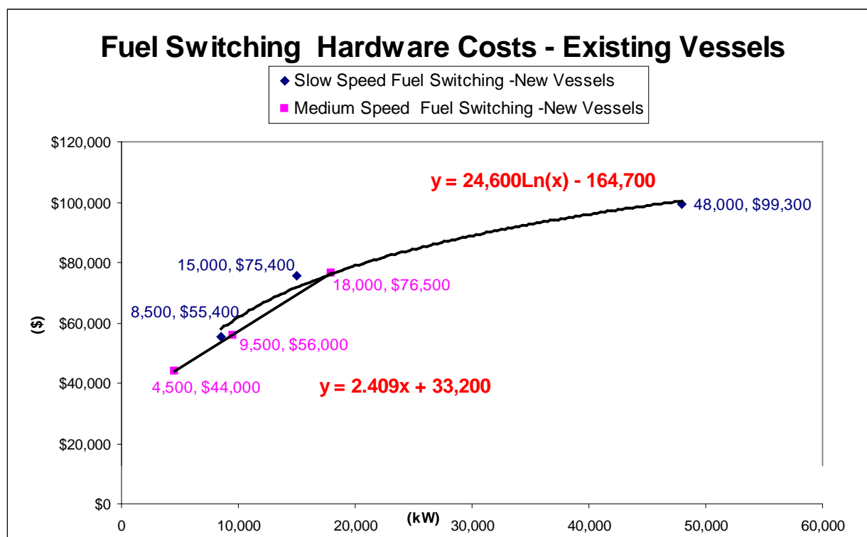
Figure 6-4 Variable Cost Curve Fit for Fuel Switching Vessels Costs to Existing Vessels
