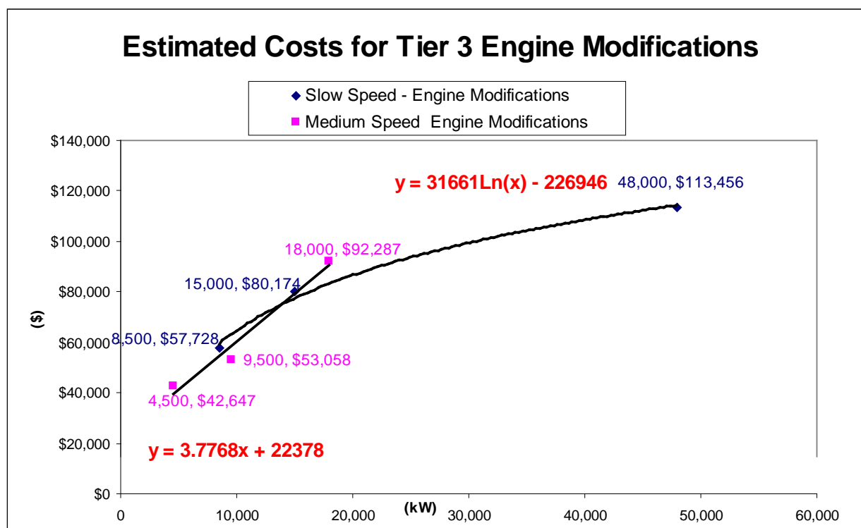
Figure 6-6 Variable Cost Curve-Fit for Engine Modifications Associated with Tier 3
