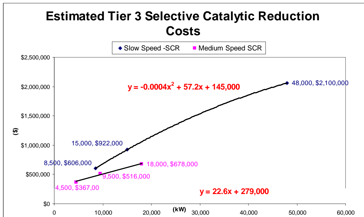
Figure 6-7 Variable Cost Curve-Fit for SCR Systems
