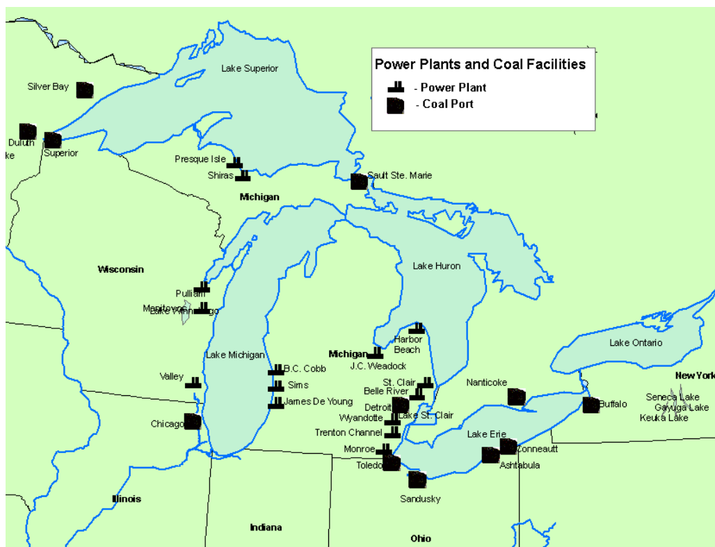
Figure 7-7 Major Great Lakes Area Coal Port Facilities and U.S. Waterside Power Plants
