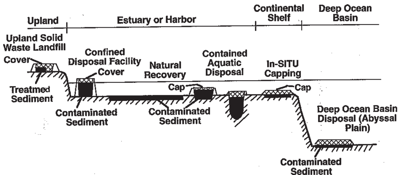
Figure 3. Conceptual illustration—containment, disposal and natural recovery technologies for contaminated bed sediments (adapted from Mike R. Palermo, USAE, Vicksburg, MS).
