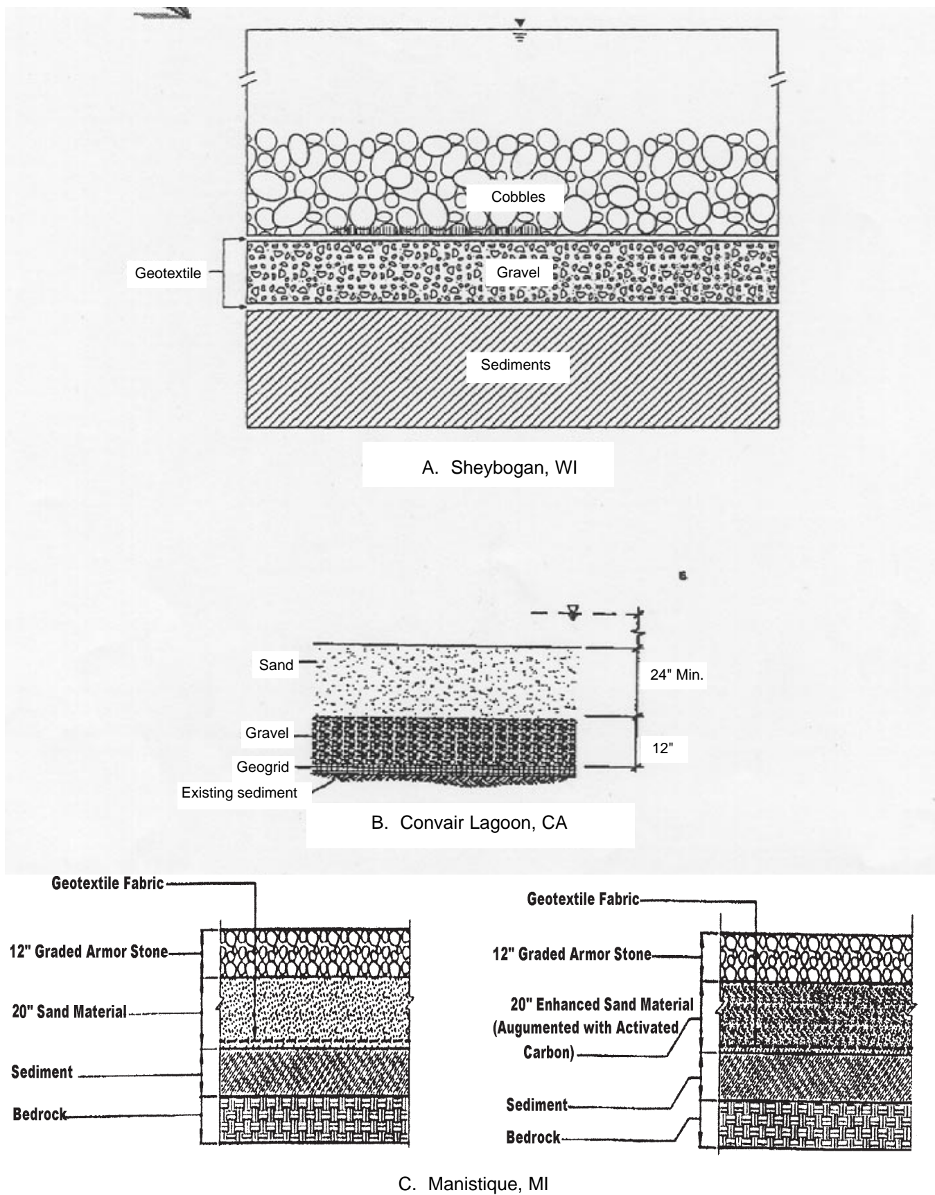
Figure 1. Illustrations of alternative combinations of cap components.
