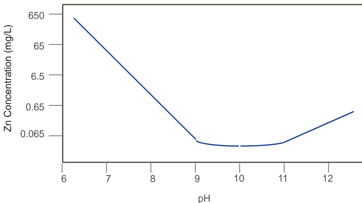
Figure 3. Zinc-contaminated site soils—zinc solubility curve.
