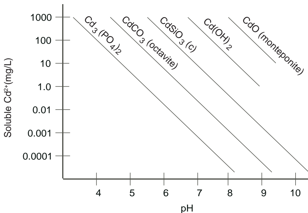
Figure 2. Solubility of cadmium species as a function of pH.
