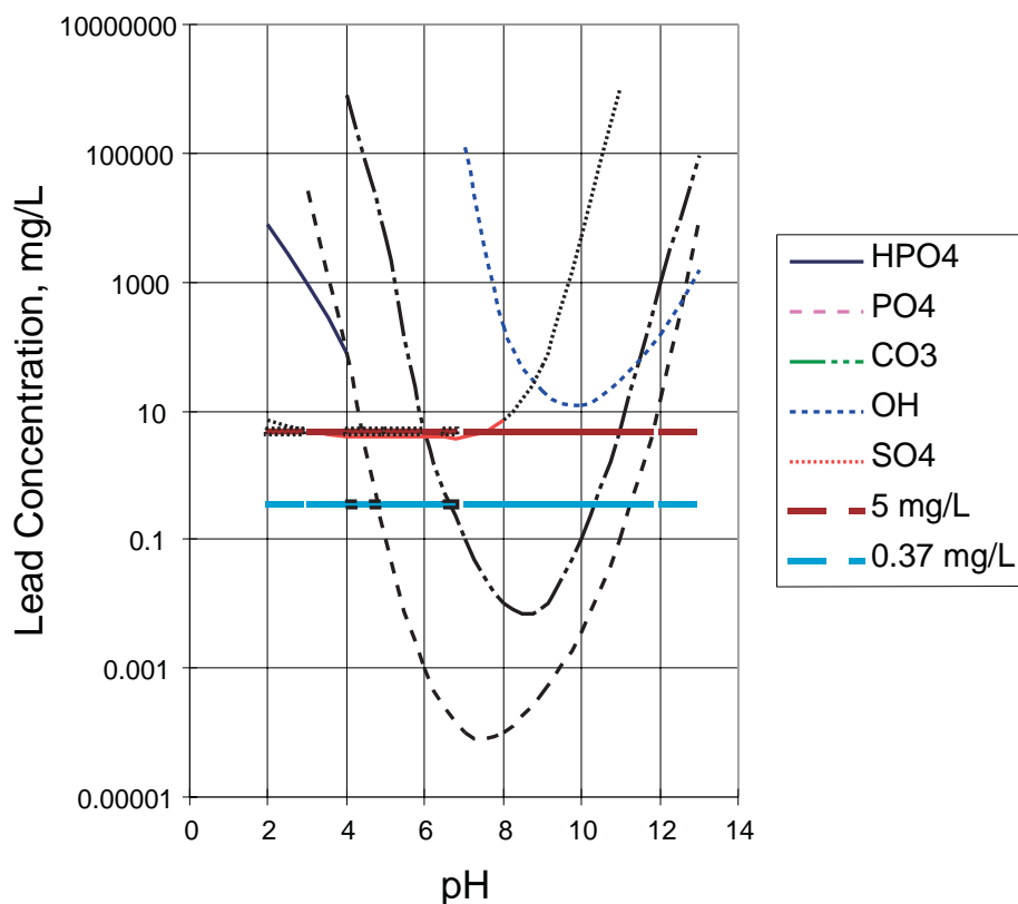
Figure 1. Solubility of lead species as a function of pH.
