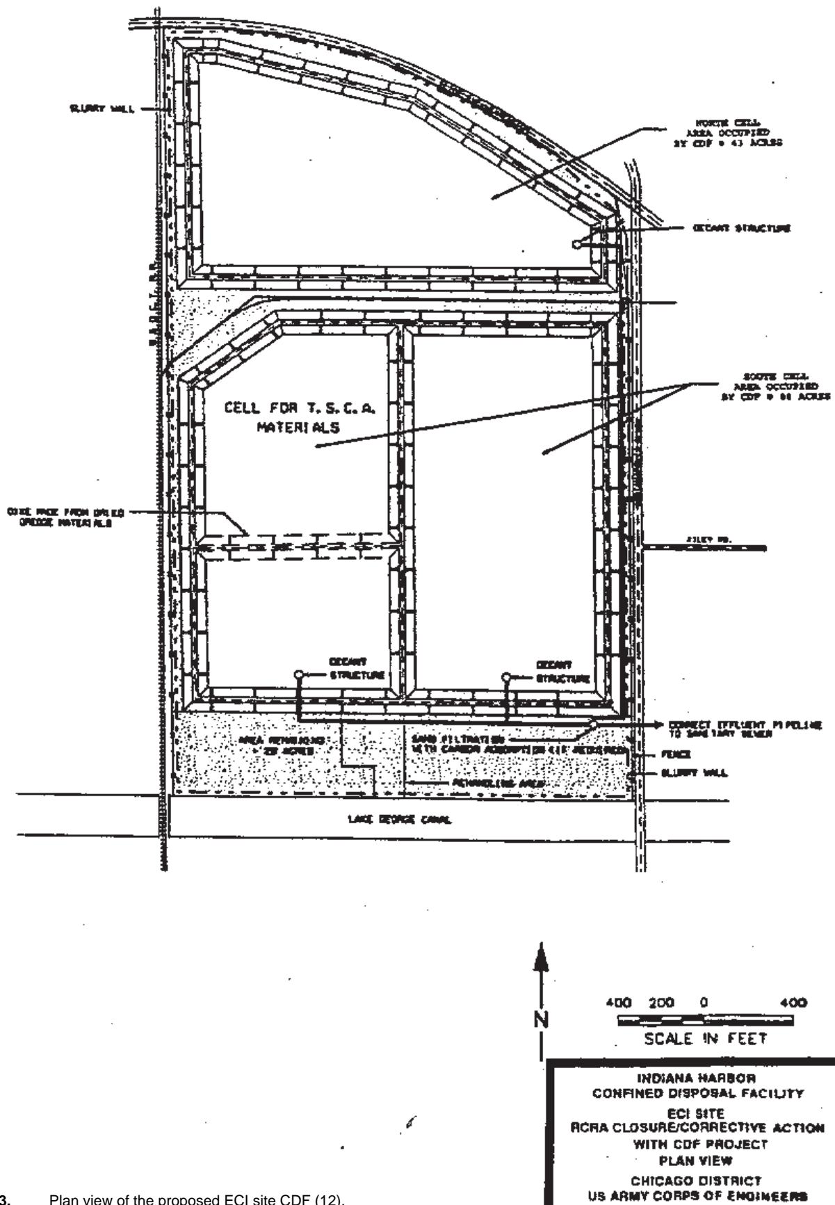
Figure 3. Plan view of the proposed ECI site CDF (12).
